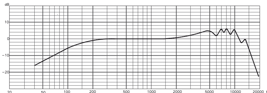
FREQUENCY RESPONSE
